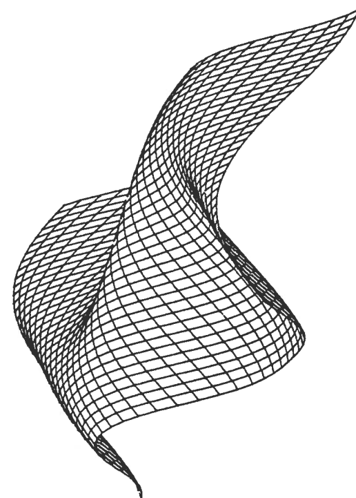
The mathematical function f(x) = \cos(y = \sin(2x)) with hidden line removal. Produced on Mr. Thorman’s computer. Similar to equation plotted for class.
